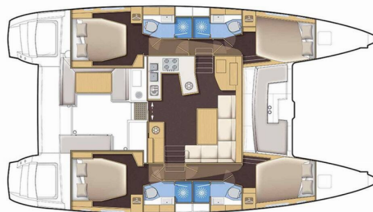
Version 4 cabines / 4 cabin version
